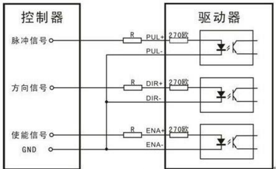
common cathode connection
