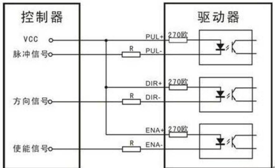
common anode connection
